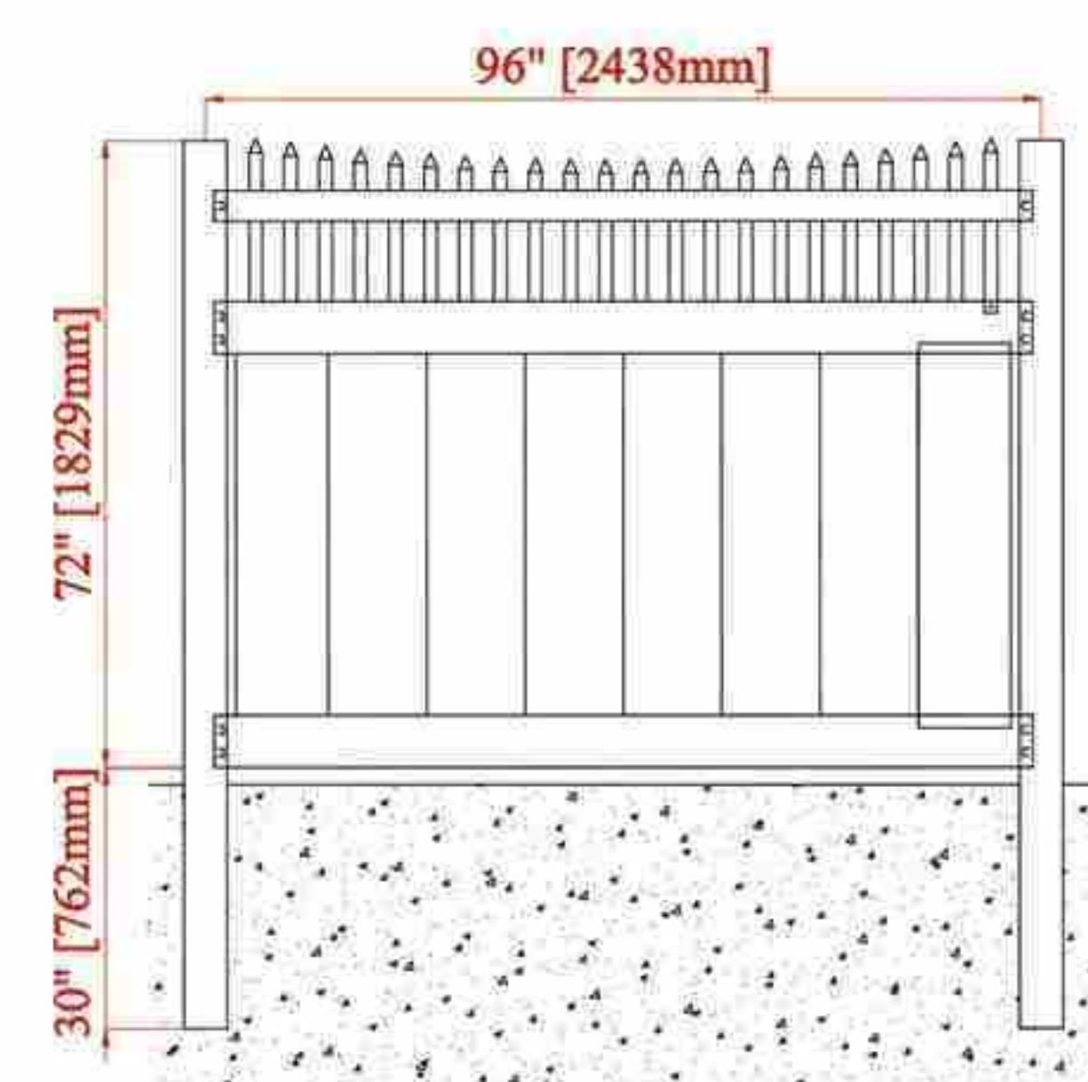
ST003 - PRIVACY FENCE WITH SCALLOPED PICKET TOP RECOMMENDED SIZE : 6' HIGH X 8' WIDE
