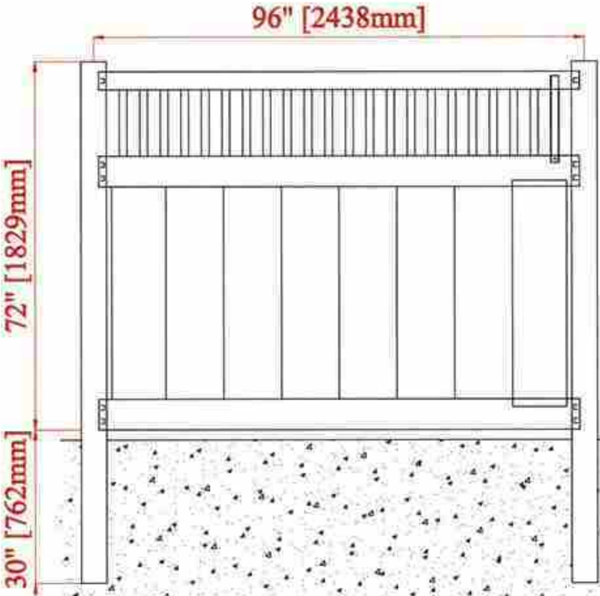
ST004 - PRIVACY FENCE WITH CLOSED PICKET TOP RECOMMENDED SIZE : 6' HIGH X 8' WIDE
