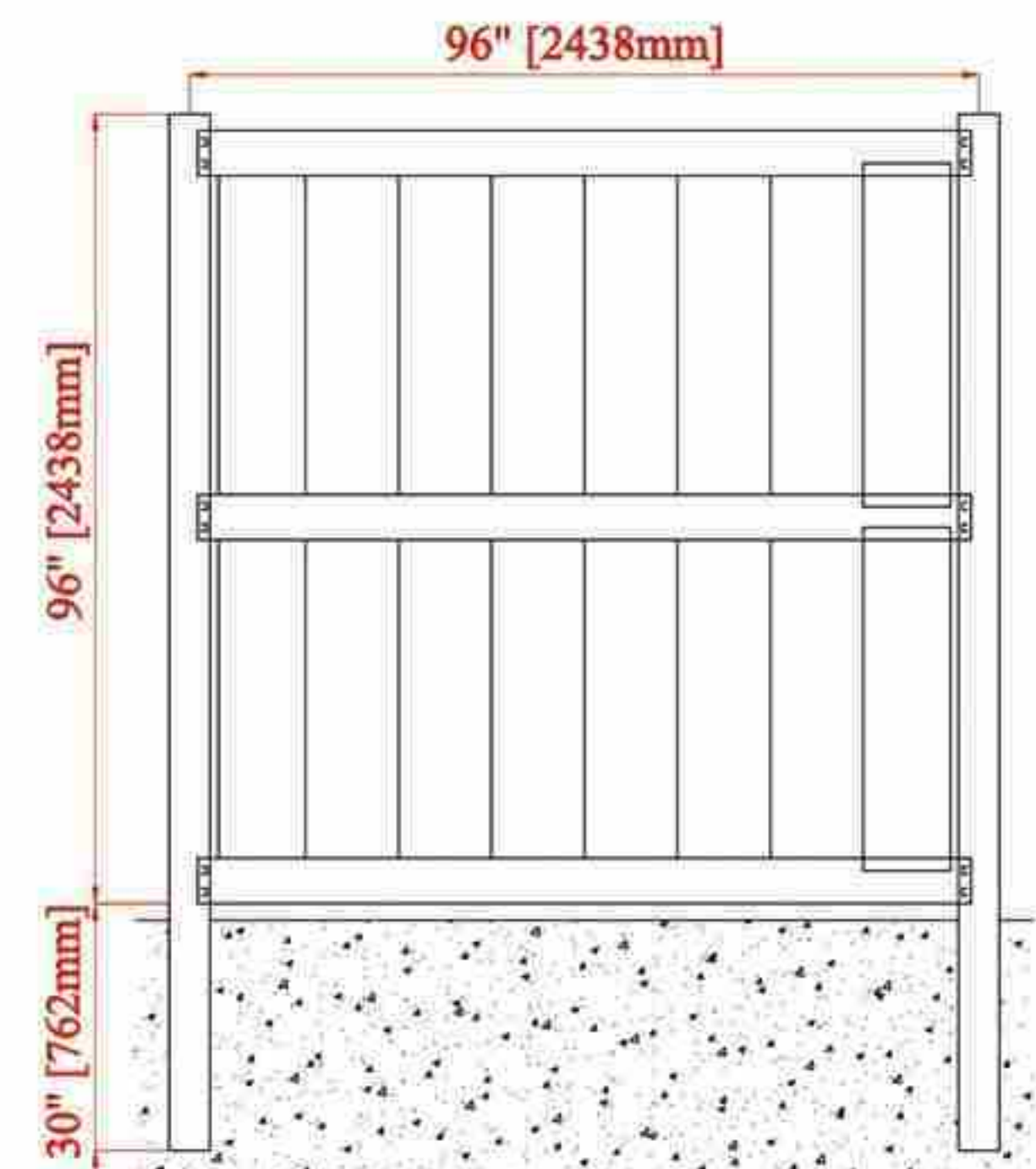
ST006 - HIGH PRIVACY FENCE RECOMMENDED SIZE : 8' HIGH X 8' WIDE
